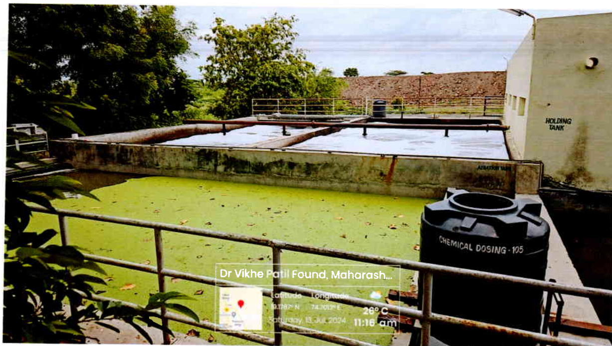
Aeration Tank and Holding
